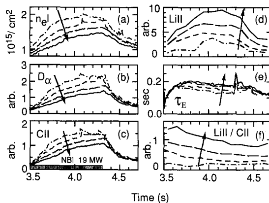
Fig. 1. Time variation of n_e l , D_\alpha , CII, LiII, \tau_E , and the ratio of LiII/CII for different levels of conditioning. Some operating parameters for the four shots: P_b = 19.5 MW, I_p = 2.48 MA, B_\phi = 5.1 T, and R_p = 2.52 m. Pellets injected at t \leq 2.7 s. No-Li (dot-dash), 1-pellet (short-dash), 2-pellet (long-dash), 3-pellet (solid).
