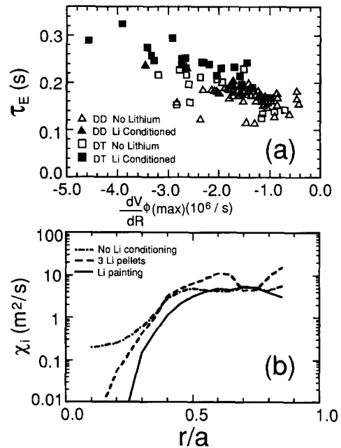
Fig. 5. (a) \tau_E versus \nabla V_\phi for a wide variety of Li conditioned and no Li plasmas. (b) \chi_i for the no Li, 3 pellet Li conditioned and Li painted plasmas.
