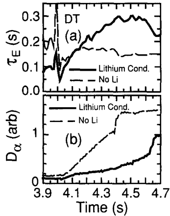
Fig. 3. \tau_E and D_\alpha signals for a high performance plasma obtained using the Li painting (solid curve) technique compared to signals without Li (dashed curve).
