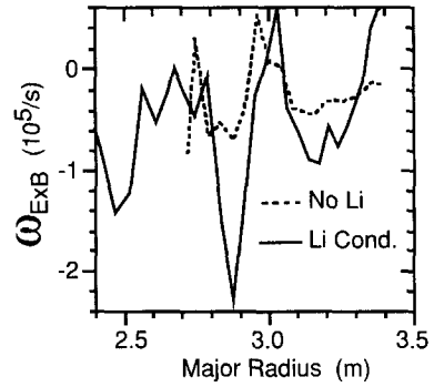
Fig. 4. Shearing rate, \omega_{E \times B} , for the Li conditioned case of Fig. 3 (solid) and the no-Li case of Fig. 2.
