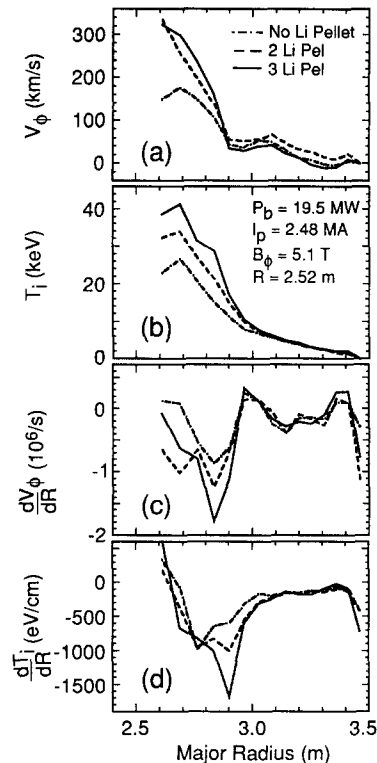
Fig. 2. Variation of V_\phi , T_i , \nabla V_\phi and \nabla T_i with Li conditioning, from no Li to 3 Li pellets.
